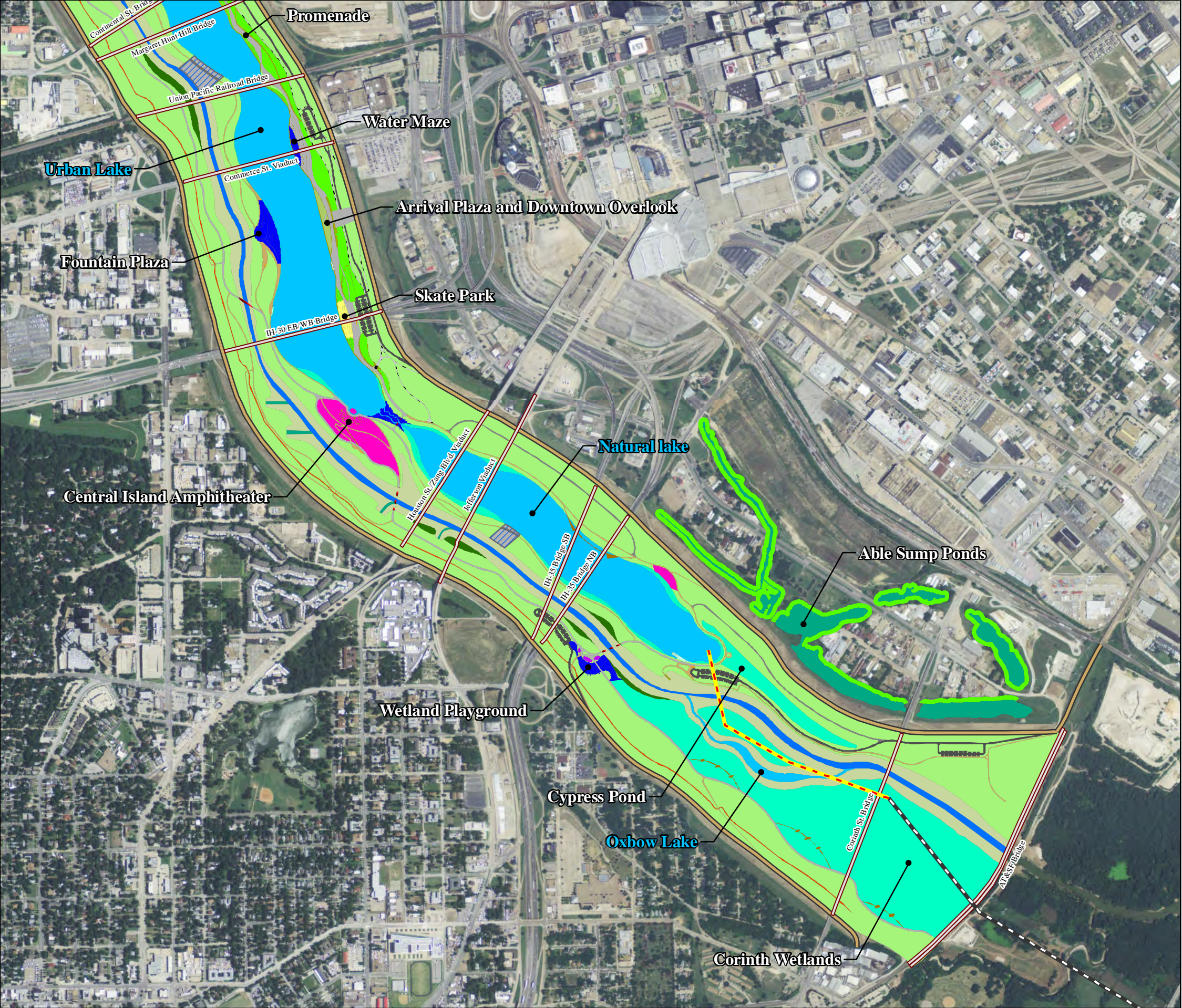
Figure 2-8 Proposed BVP Study Ecosystem and Recreation Features: Southern Segment
