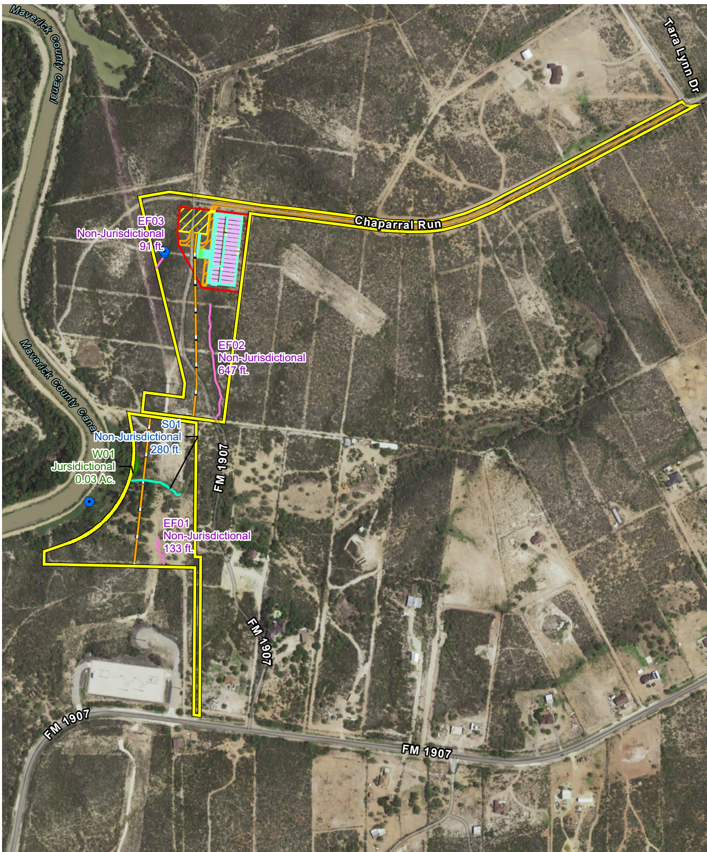
Figure 1 Site Layout & Delineation Results
