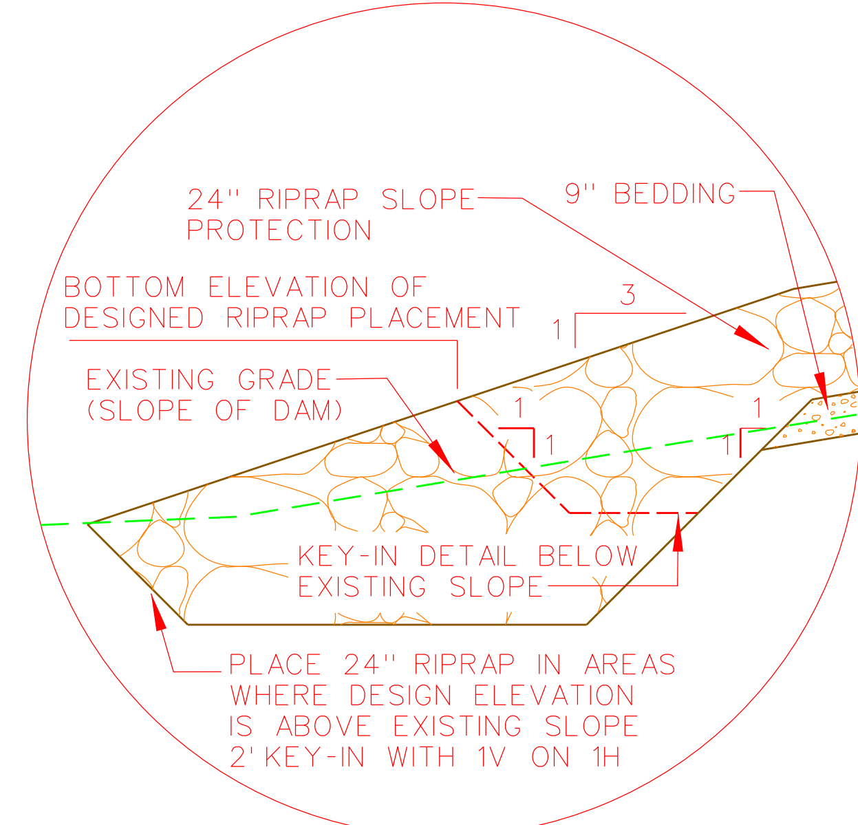
INSET "A" BOTTOM ELEVATION OF RIPRAP PLACEMENT IS ABOVE EXISTING GRADE
