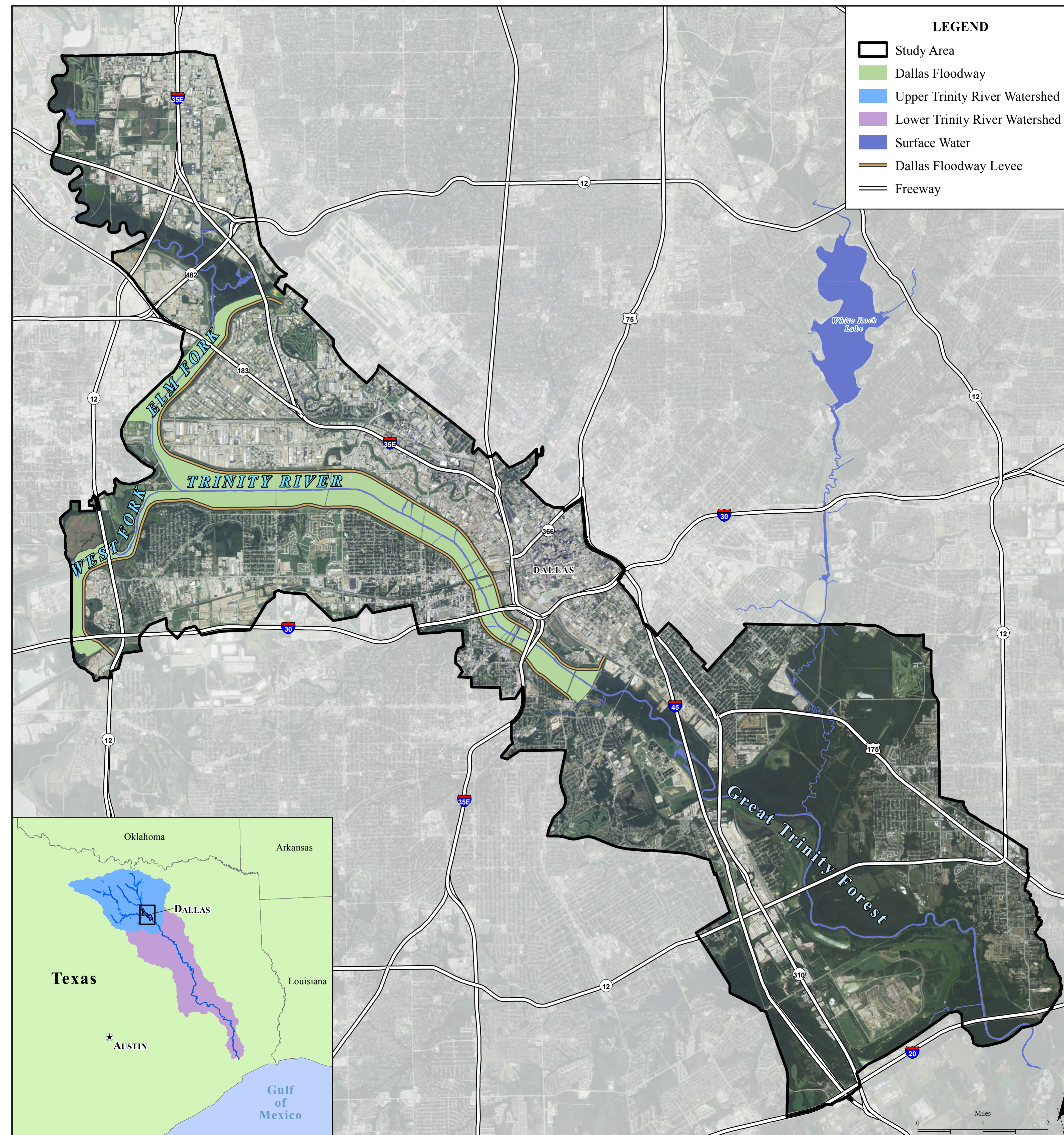
Dallas Floodway Project Environmental Impact Statement Study Area
