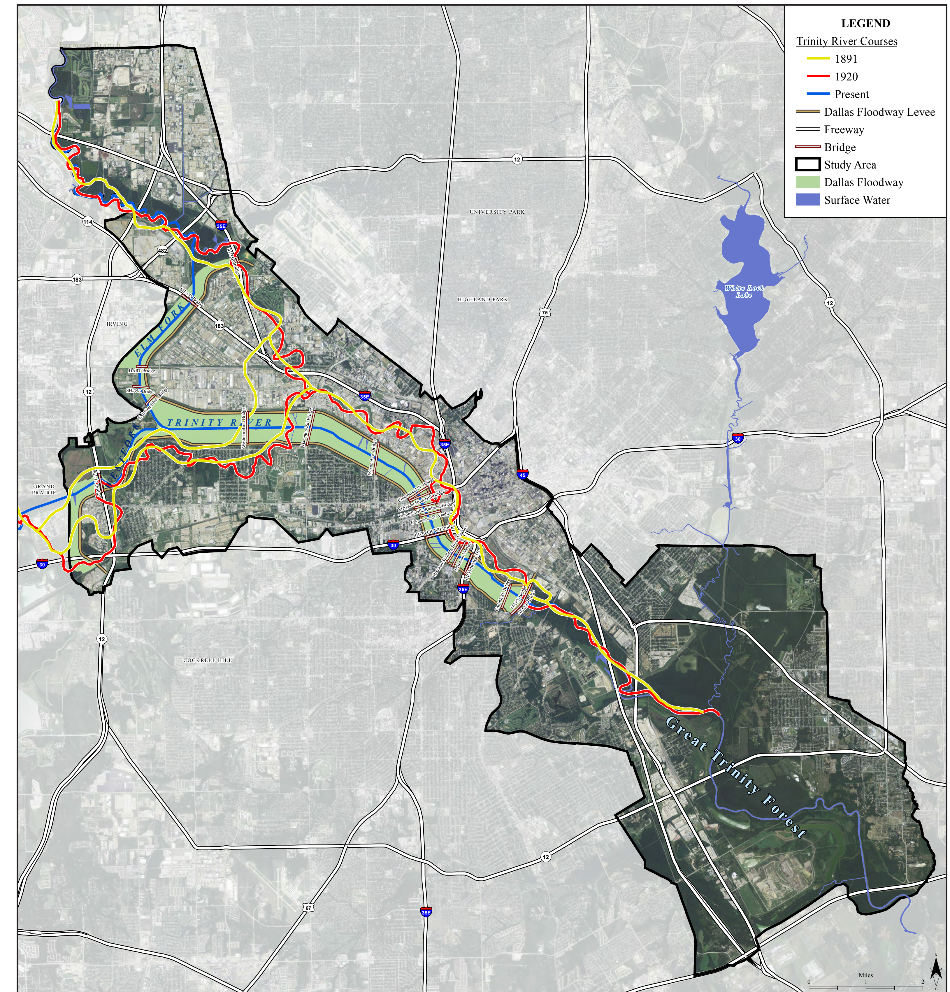
Historical and Current Trinity River Courses
