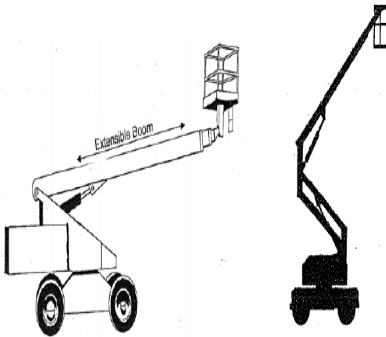
Figure 3 Boom-Supported Elevating Work Platform
